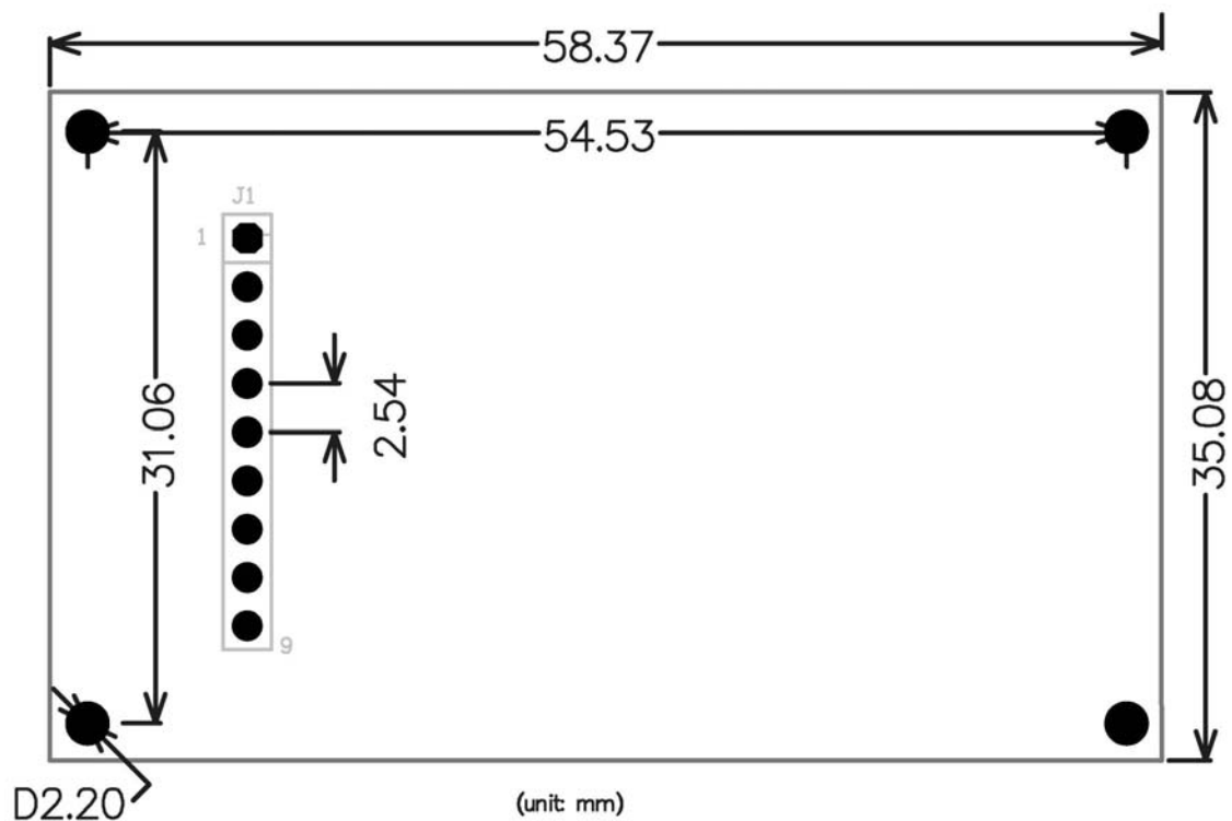
Figure 3– YHY522R Top view size
